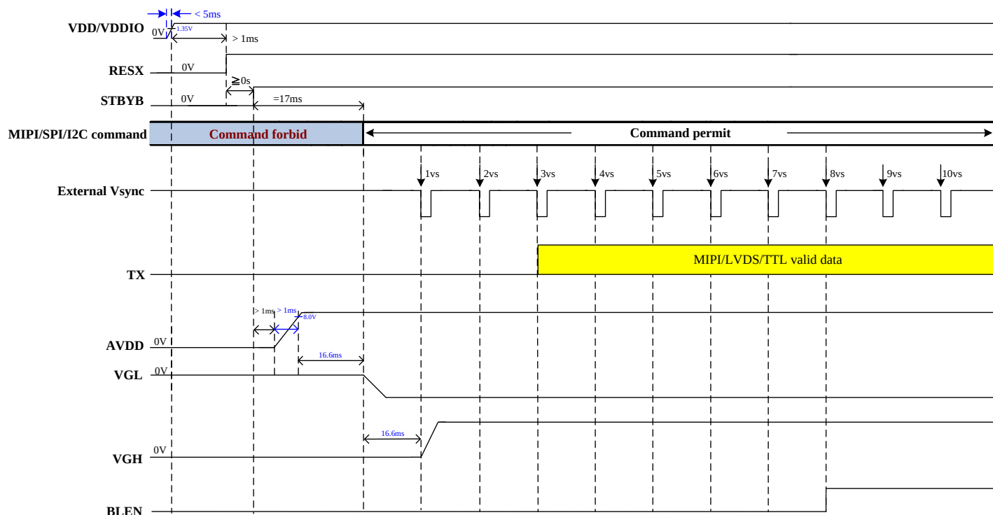
Figure : Power On timing chart
