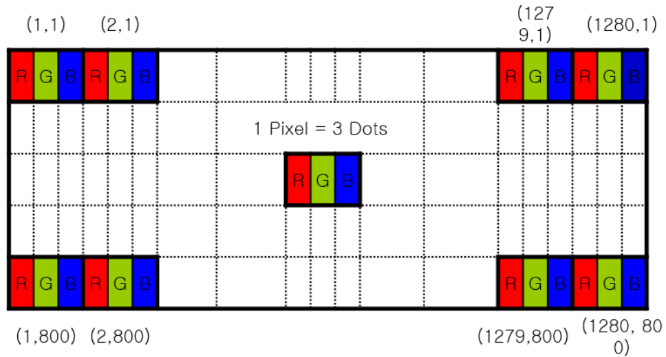
Figure 5. Pixel Format
