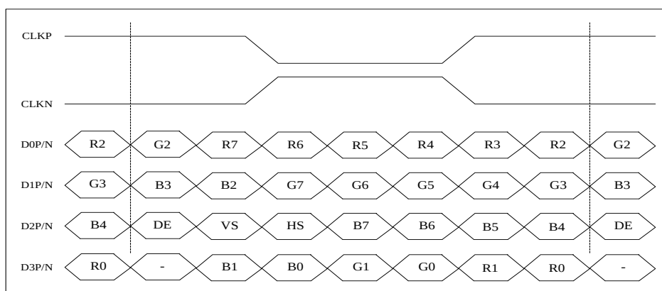
Figure 7.3: 8-bit RGB LVDS JEIDA input timing
