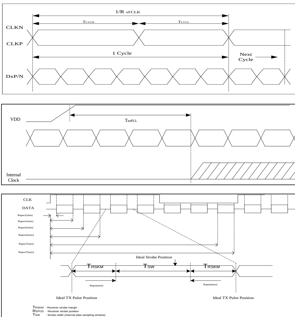
Figure 7.4: LVDS figure
