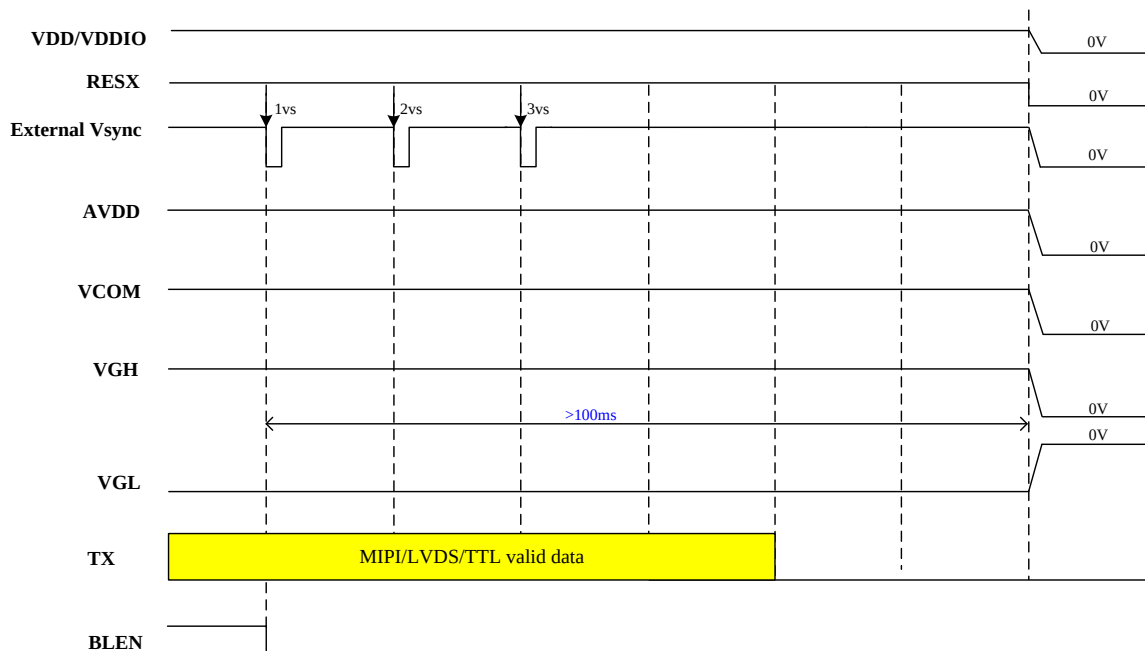
Figure : Power Off timing chart
