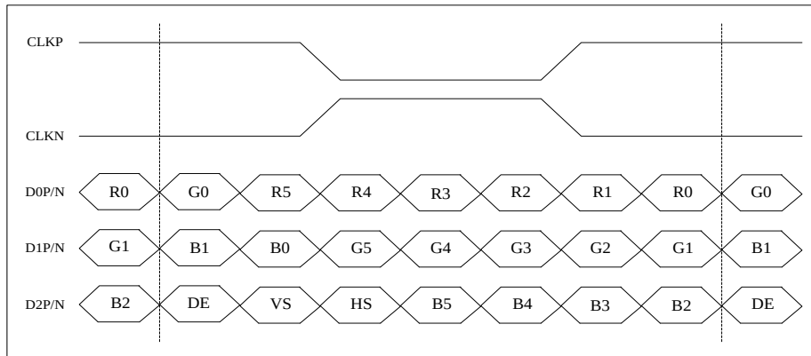
Figure 7.1: 6-bit RGB LVDS input timing
