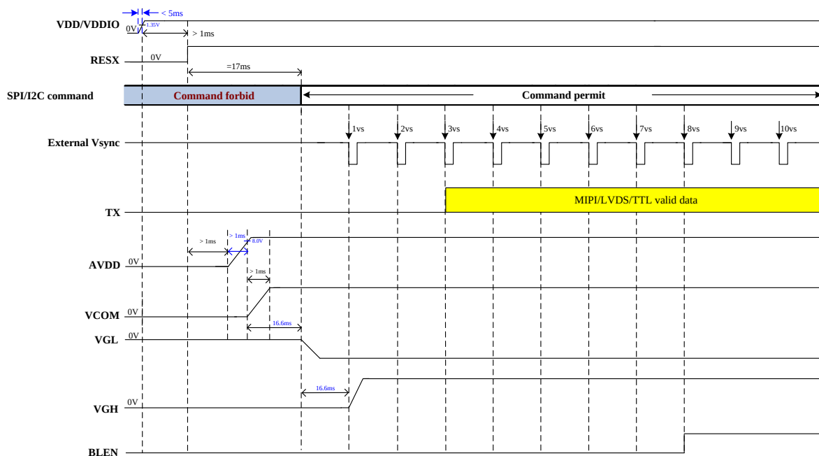
Figure : Power On timing chart
