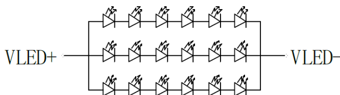
BL CIRCUIT DIAGRAM V_F=18.6V (TYP) , I_F=60mA
