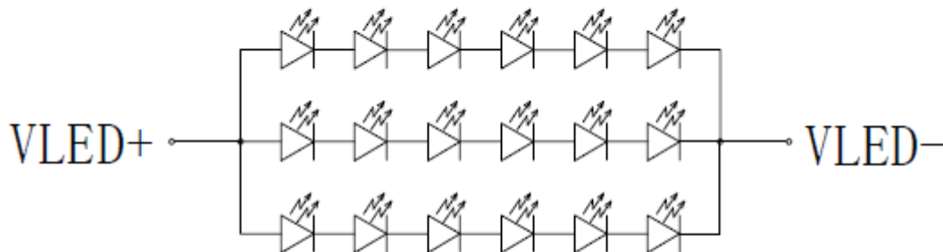
BL CIRCUIT DIAGRAM V_F = 18.6\text{V} (TYP) , I_F = 60\text{mA}
