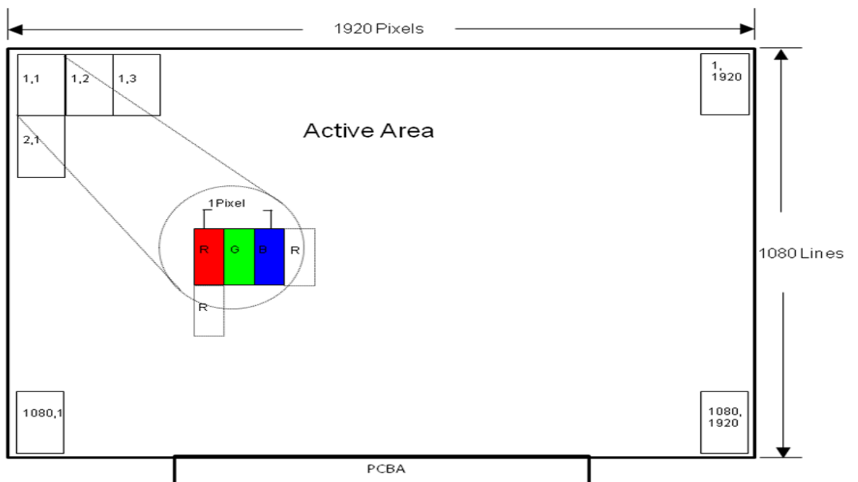
Figure 2 Pixel Mapping
