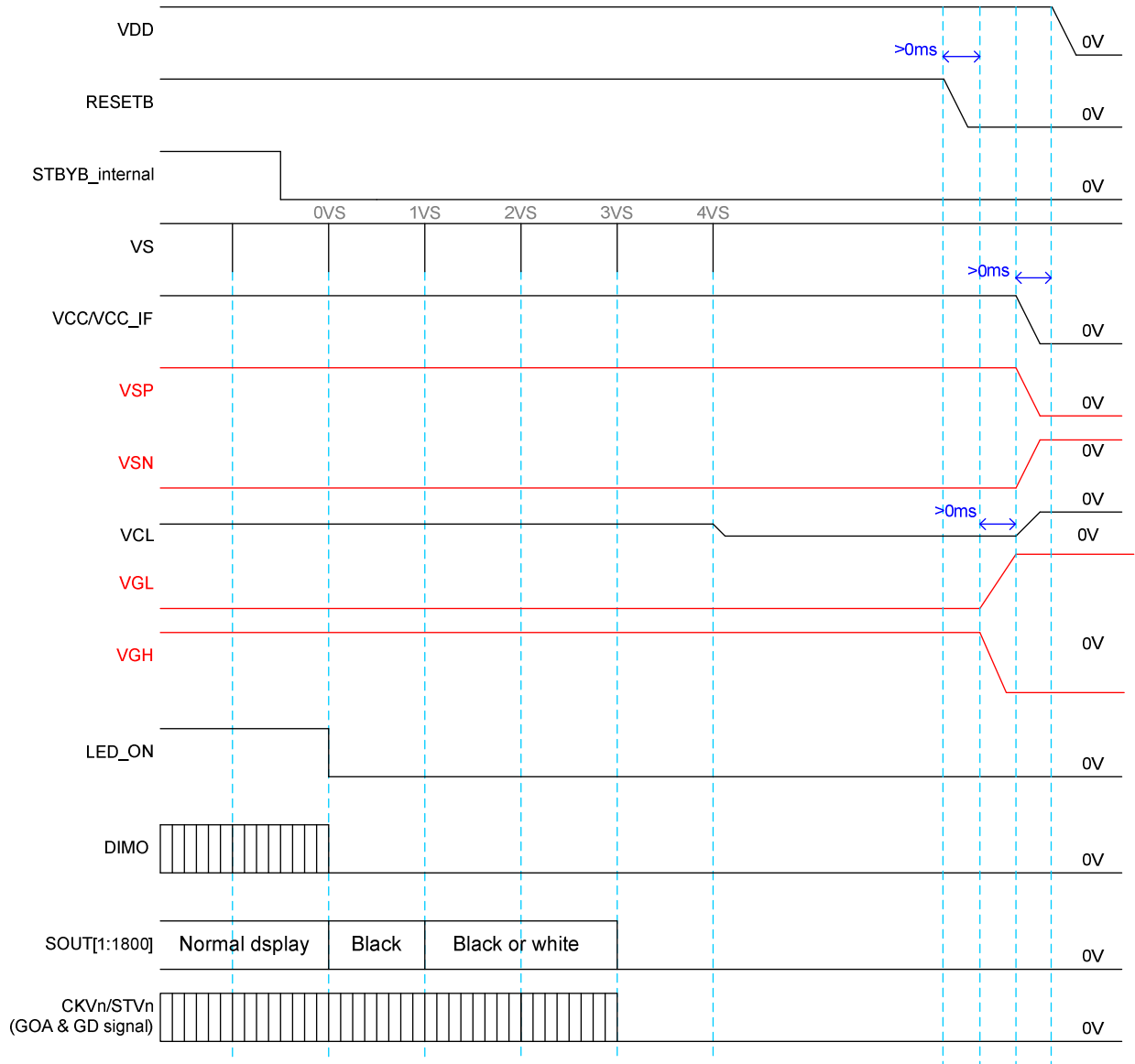
Figure 5.8: Power off sequence with PWRMD=1
